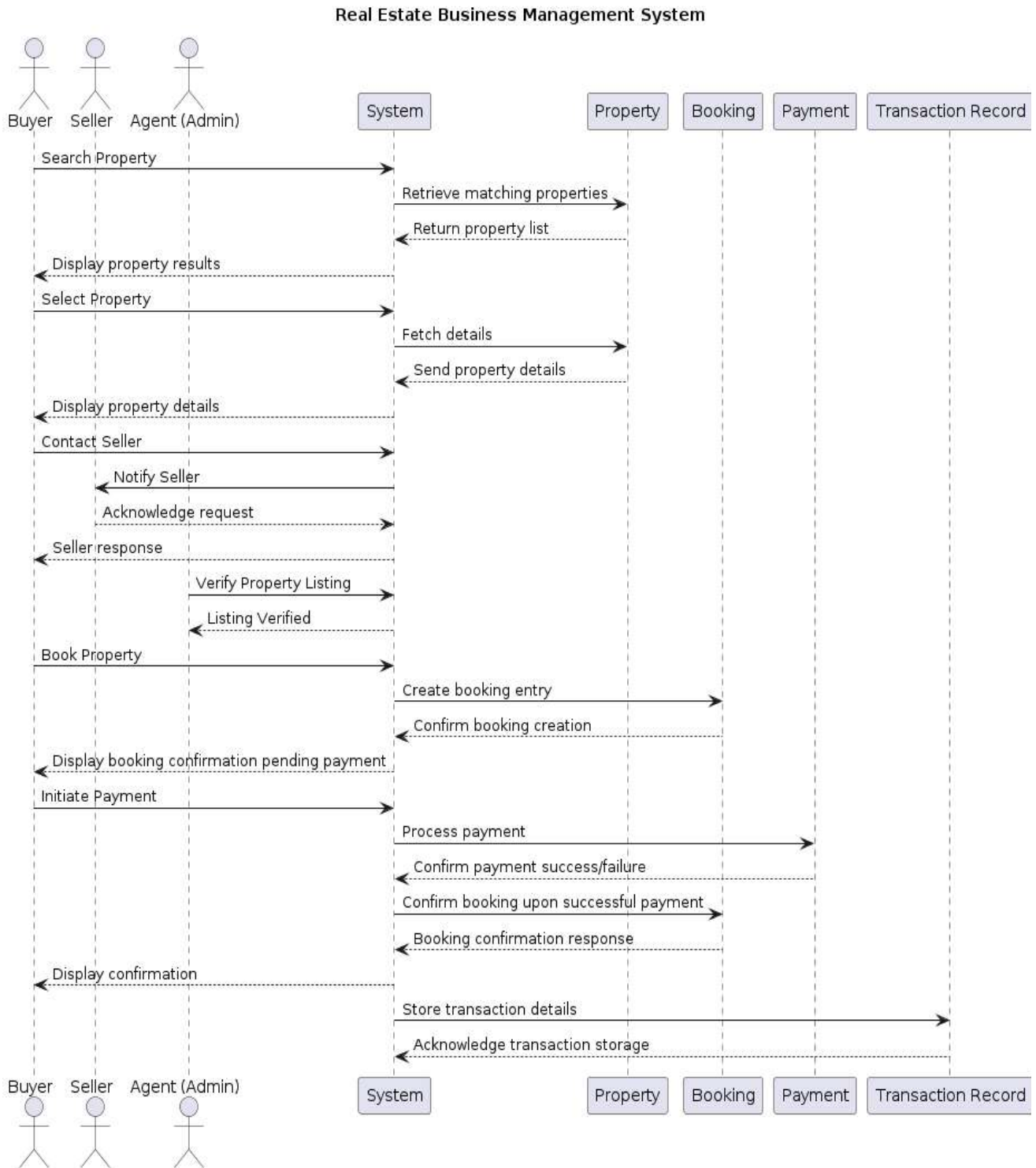
Fig 2(b): Sequence Diagram
