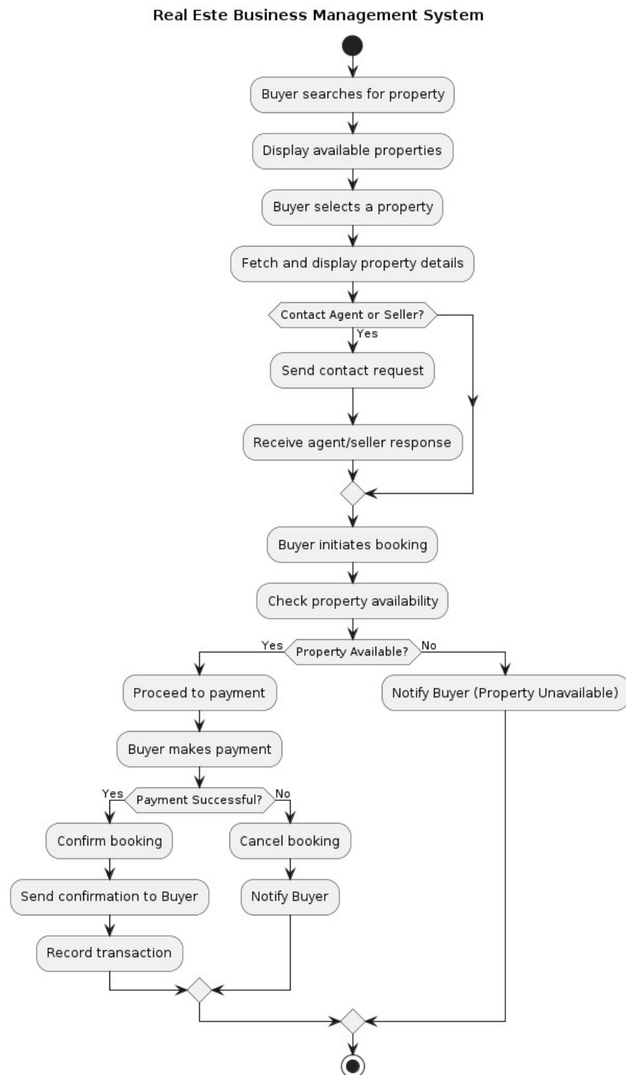
Fig 2(d): Activity Diagram
