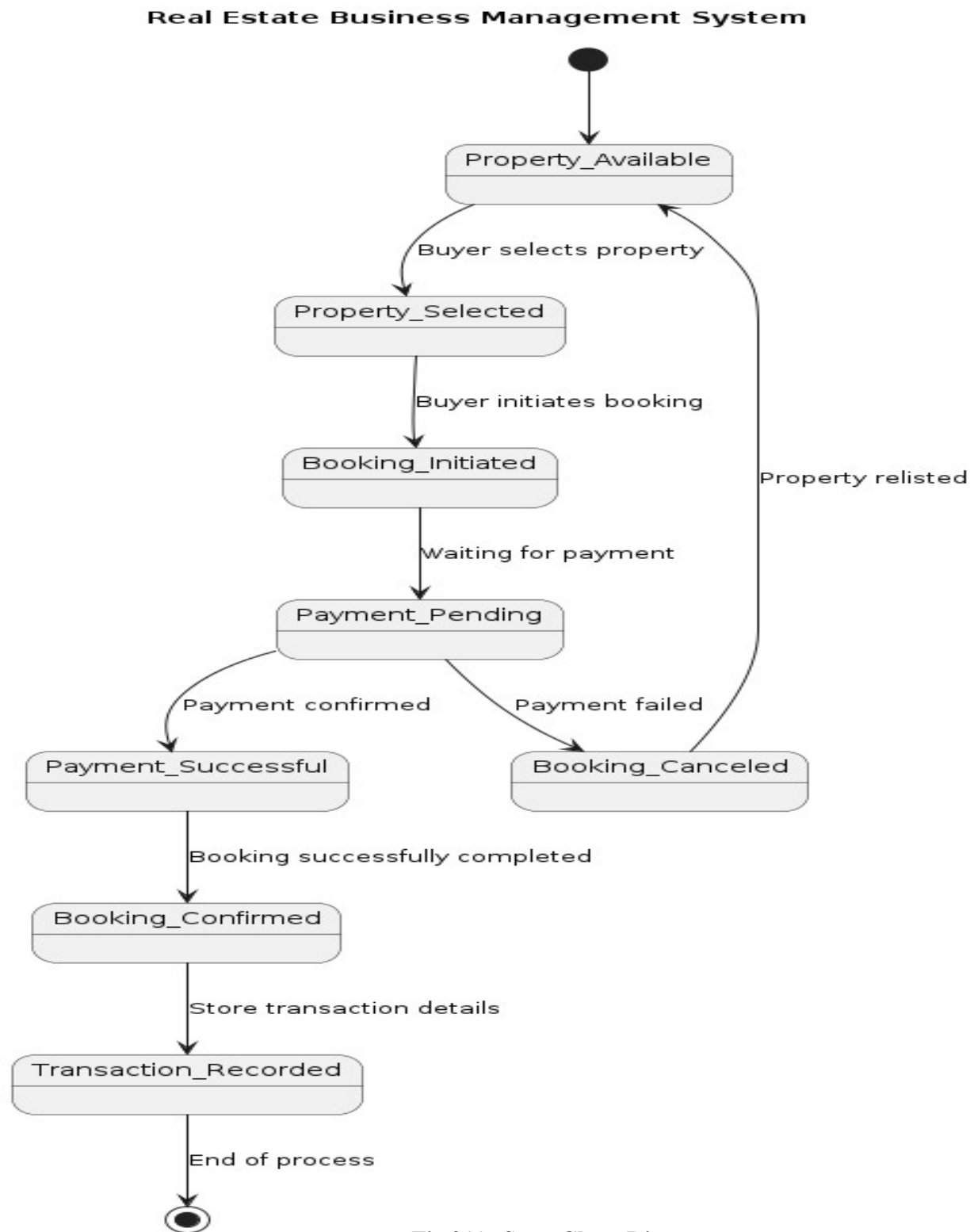
Fig 2(c): State Chart Diagram
