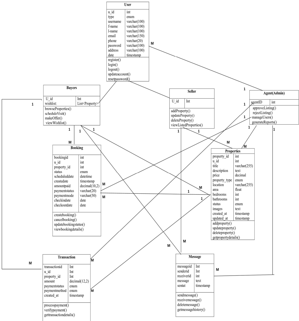
Fig 2(a): Class Diagram
